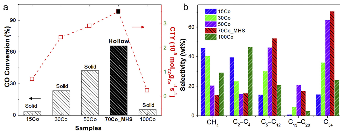
Fig. 5. a) CO conversion (black, column) and cobalt-time-yield CTY (red, square) of the Co 3 O 4 -Al 2 O 3 samples; b) Products selectivity of the Co 3 O 4 -Al 2 O 3 samples. Reaction conditions: TOS = 5 h, H 2 /CO = 2/1, T = 220 °C, 2 MPa, GHSV = 7500 mL g -1 h -1 . (For interpretation of the references to colour in this figure legend, the reader is referred to the web version of this article.)
