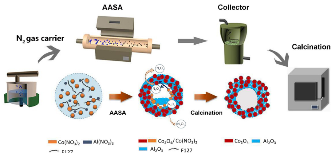
Scheme 1. Schematic illustration on the stepwise formation of \text{Co}_3\text{O}_4\text{-Al}_2\text{O}_3 MHS.
