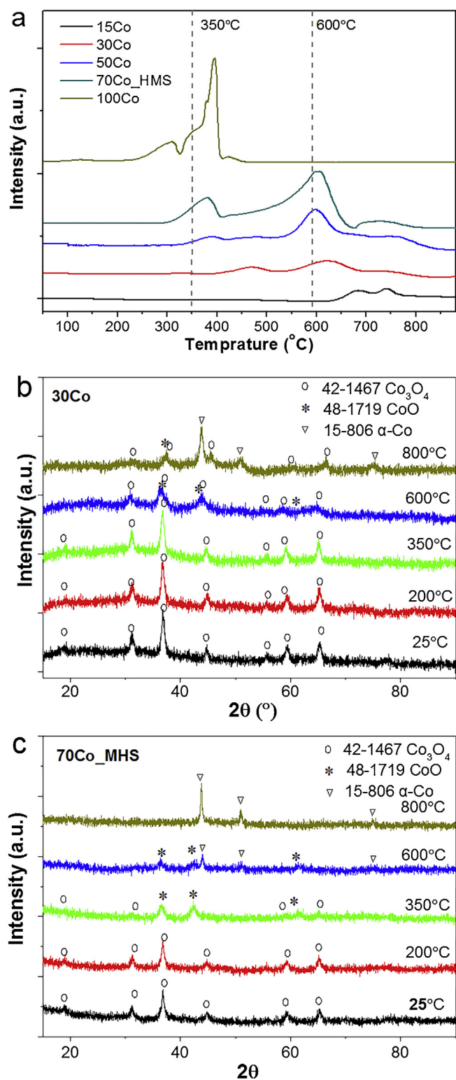
Fig. 11. a) H 2 -TPR profiles of the Co 3 O 4 /Al 2 O 3 samples; In-situ XRD patterns of b) 30Co and c) 70Co_MHS under the same testing conditions as H 2 -TPR.
