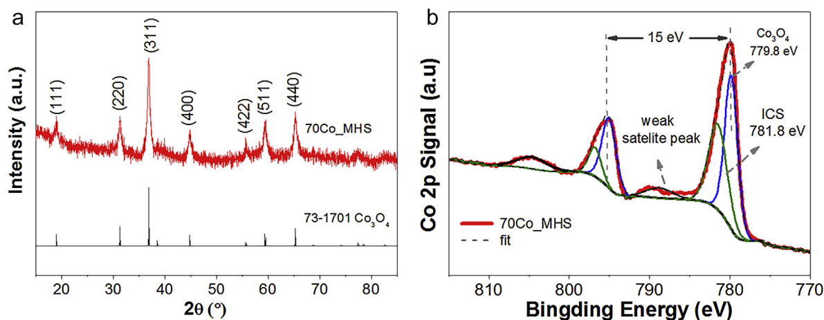
Fig. 2. a) XRD pattern and b) Co 2p XPS profile of as prepared 70Co.MHS.
