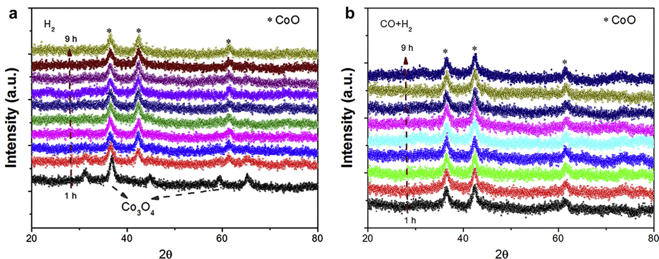
Fig. 10. In-situ XRD patterns of 70Co.MHS during various condition: a) 10% H 2 /Ar, 50 mL/min, 350 °C. b) 33.3% CO/H 2 , 15 mL/min, 220 °C.
