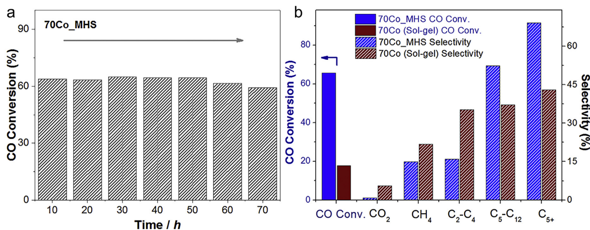
Fig. 6. a) Long-time test on 70Co_MHS. b) Catalytic performance of 70Co_MHS and 70Co (Sol-gel). Reaction conditions: TOS = 5 h, H 2 /CO = 2/1, T = 220 °C, 2 MPa, GHSV = 7500 mL g -1 h -1 .
