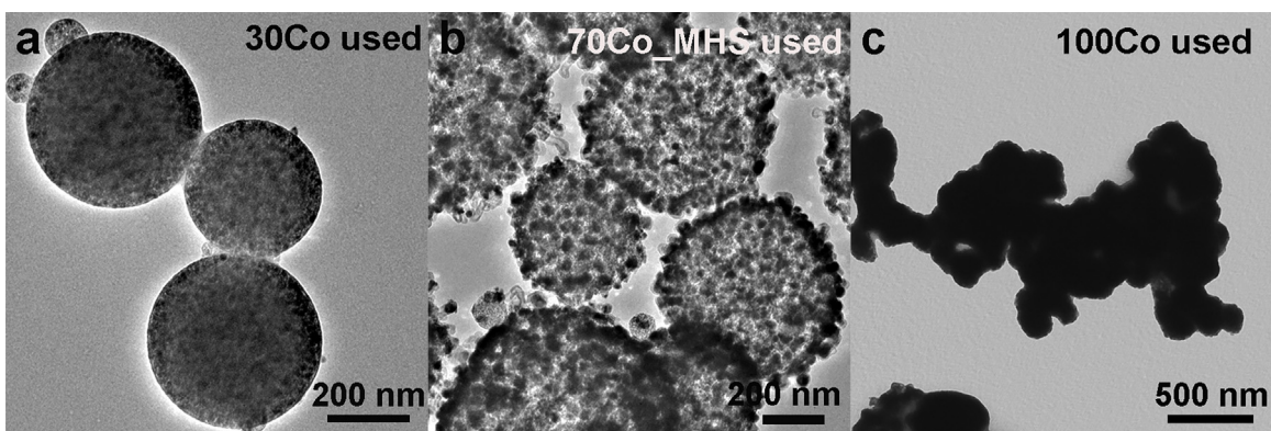
Fig. 7. TEM images of catalysts after FTS reaction. a) 30Co used, b) 70Co_MHS used and c) 100Co used.
