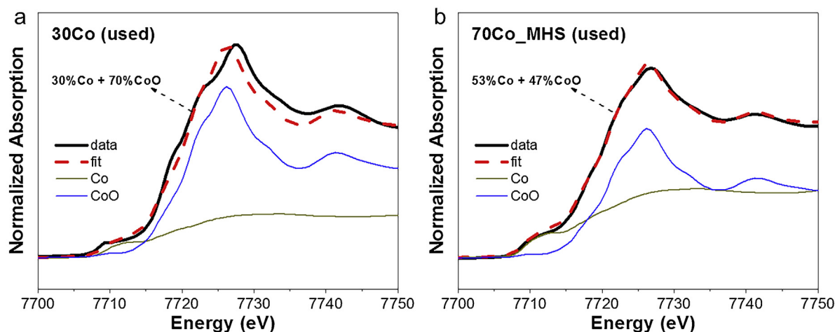
Fig. 9. XANES liner combination fits on a) 30Co (used) and b) 70Co.MHS (used).
