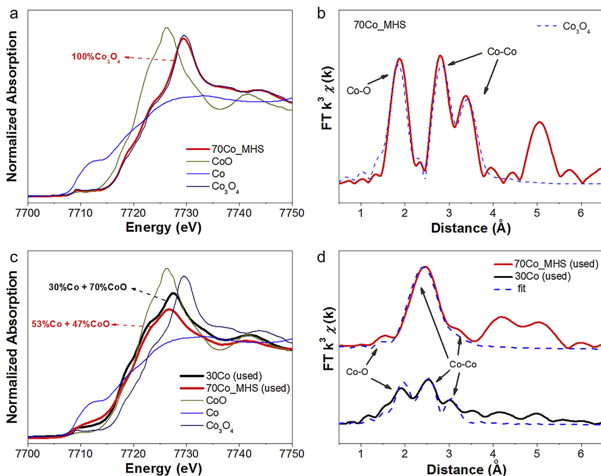
Fig. 8. a,c) XANES profile and b,d) EXAFS spectra with fitting curves in R space for the \text{Co}_3\text{O}_4\text{-Al}_2\text{O}_3 samples a,b) before and c,d) after FTS.
