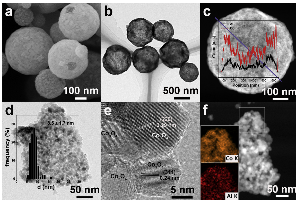
Fig. 1. a) SEM image, b) TEM image and c) STEM-EDS elemental line scanning of as-prepared 70Co.MHS; d) TEM image (inserted is the statistical histogram on particle size), e) HRTEM image and f) STEM-EDS elemental area mapping of crushed 70Co.MHS.
