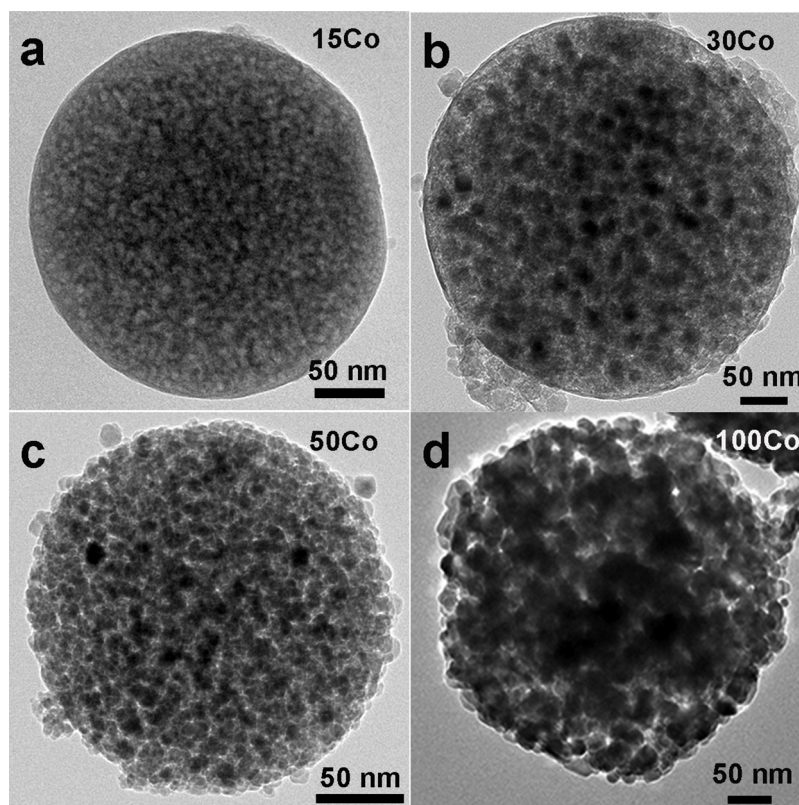
Fig. 3. TEM images of the \text{Co}_3\text{O}_4\text{-Al}_2\text{O}_3 samples: a) 15Co; b) 30Co; c) 50Co; d) 100Co.
