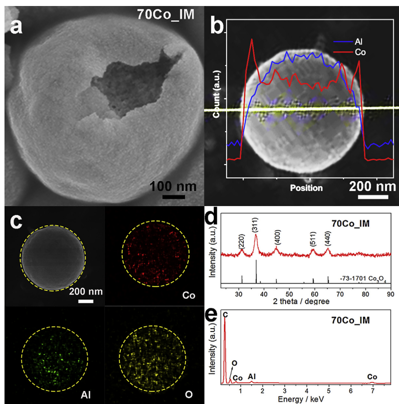
Fig. 4. a) SEM image, b) STEM-EDS elemental line scanning, c) STEM-EDS elemental area mapping and d) XRD pattern of 70Co.IM.
